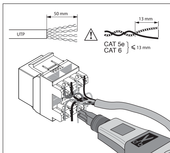
110 IDC classic connection
